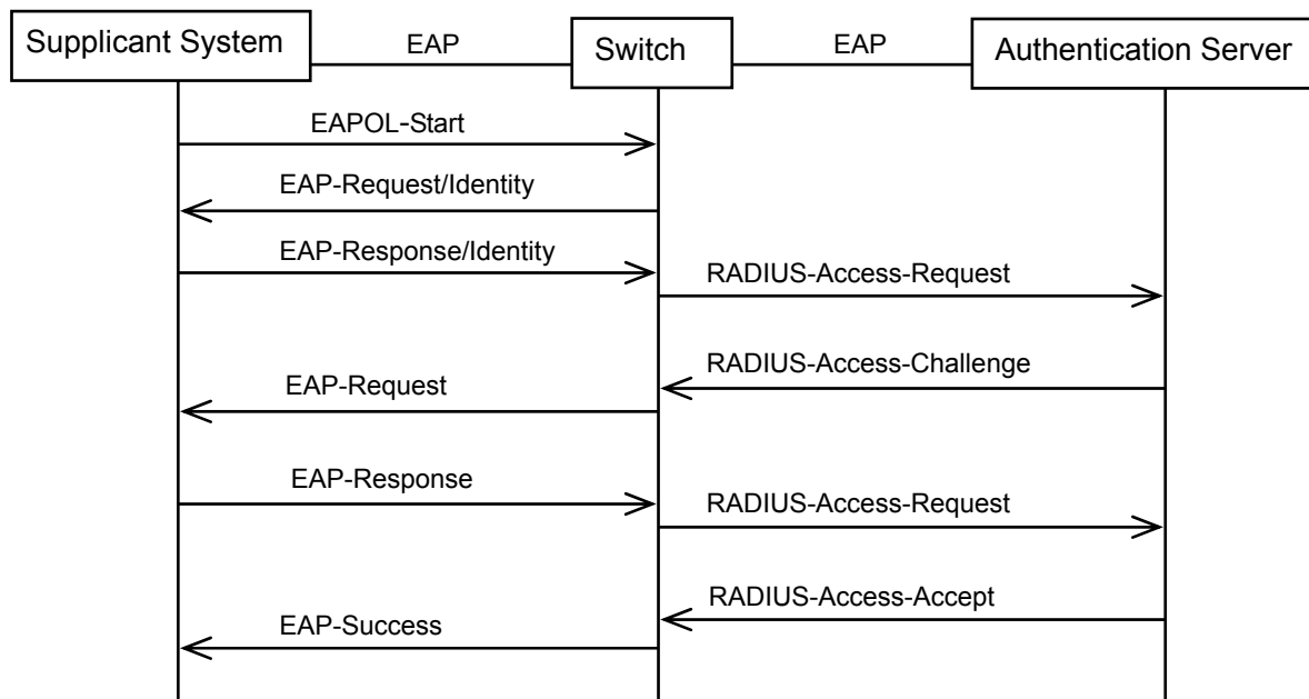
Figure 11-18 EAP-MD5 Authentication Procedure
